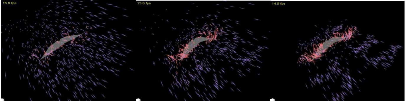
Figure 1: Particle eels turn red in low \lambda_2 regions. (a), (b) and (c) show variations of randomness in the selection of pathlines. (a) shows random selection of pathlines, (c) shows only pathlines with negative \lambda_2 .
