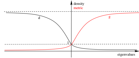
Figure 6: Example of a density function used to encode a metric
